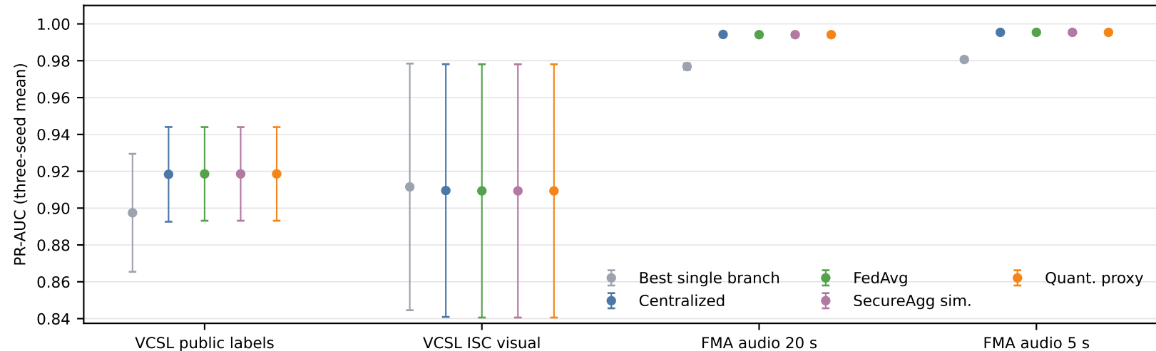
Fixed-evidence calibration across evaluation tiers
