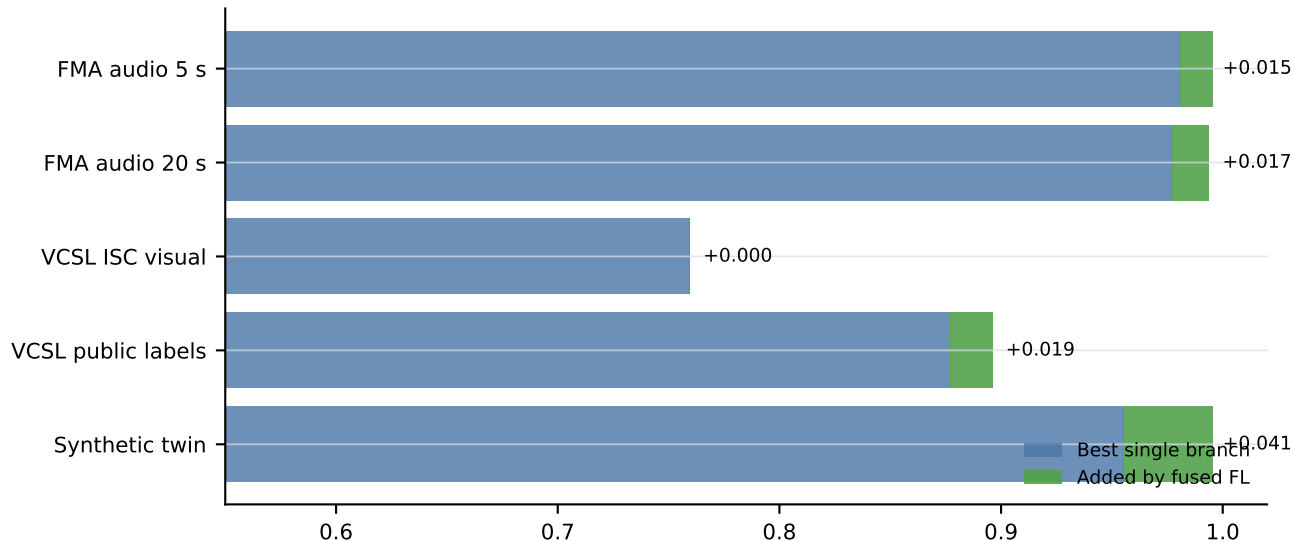
Single-branch versus fused privacy-preserving model
