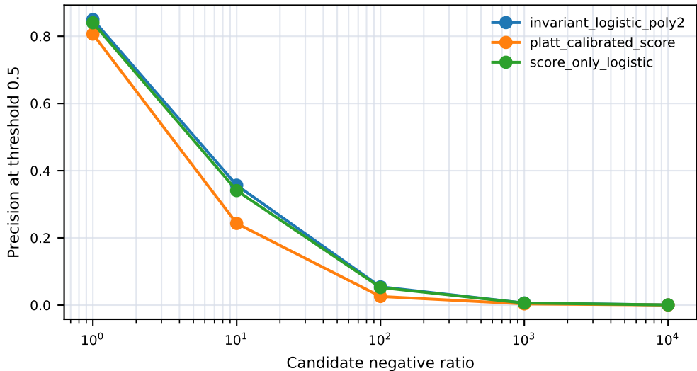
Open-set candidate-pool precision sensitivity
