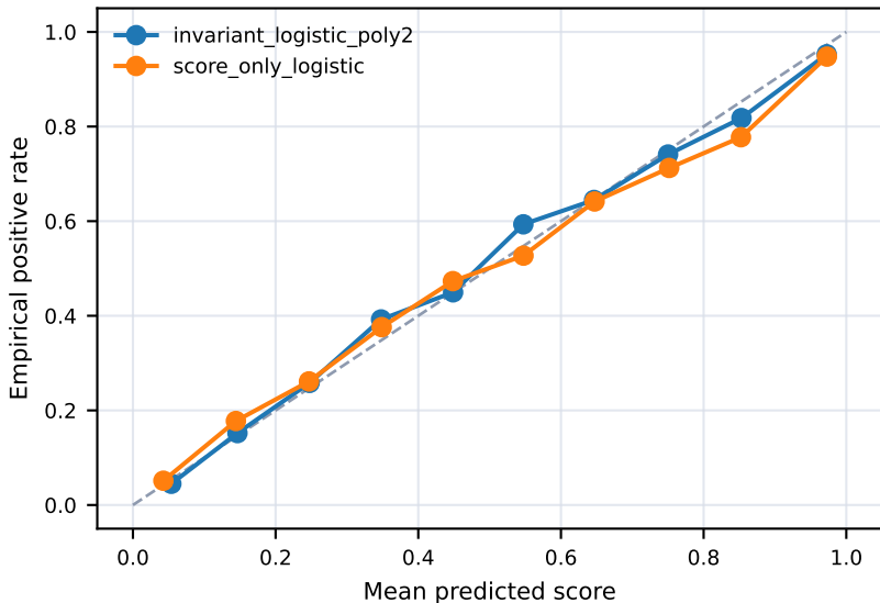
Reliability curves on VCSL public-label audit tier
