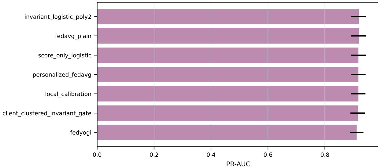
Personalization and clustered calibration on VCSL public-label audit tier
