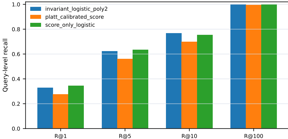
Retrieval-like ranking on VCSL public-label candidates (1:100)
