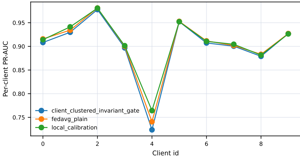
Client variability under global, local, and clustered calibration
