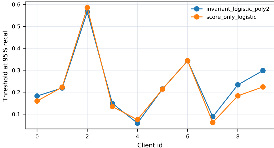
Client threshold stability diagnostic
