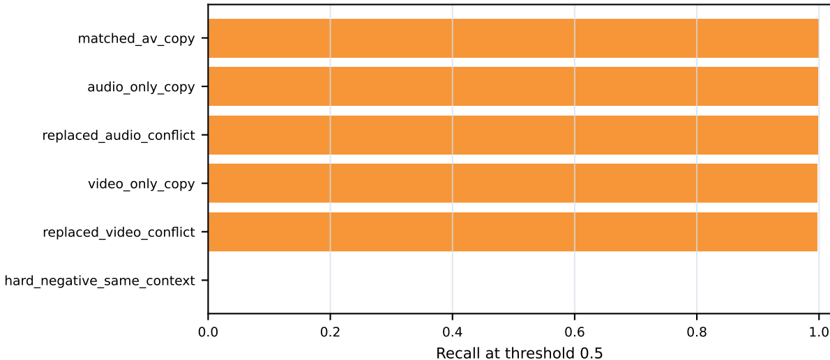
Synthetic A/V stress: scenario breakdown
