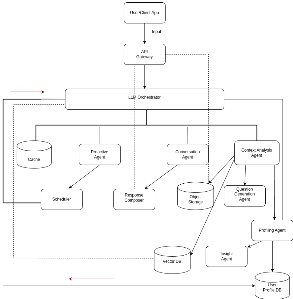
Figure 3.1: High Level Design
