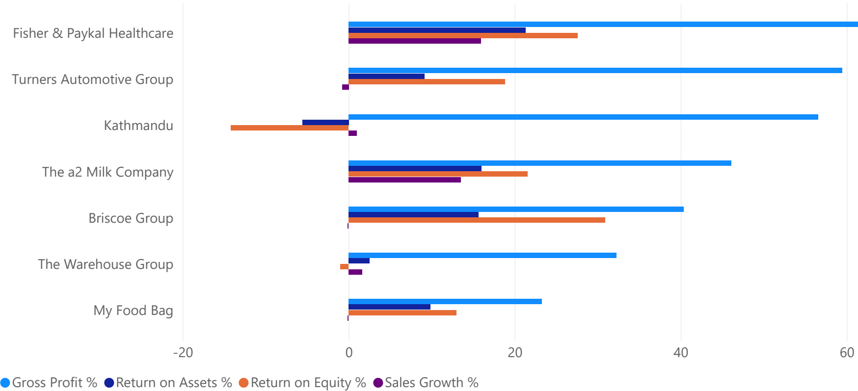
Gross Profit %, Return on Assets %, Return on Equity % and Sales Growth % by Company
