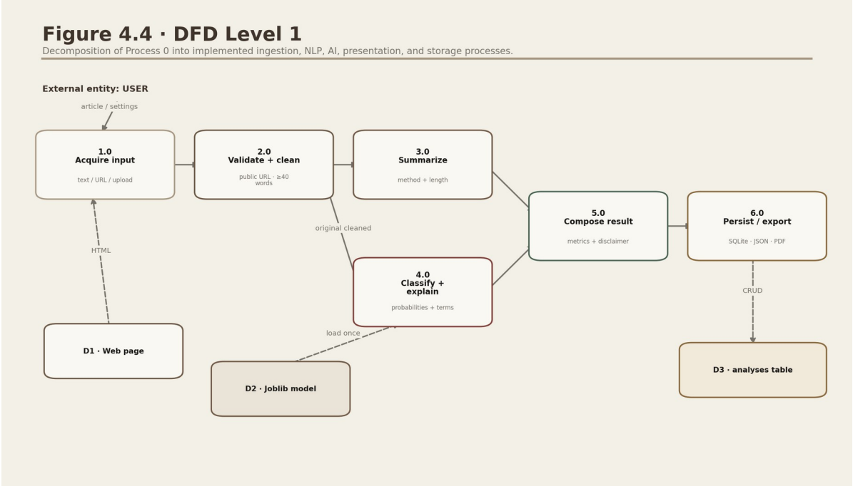
Figure 4.4. DFD Level 1.
