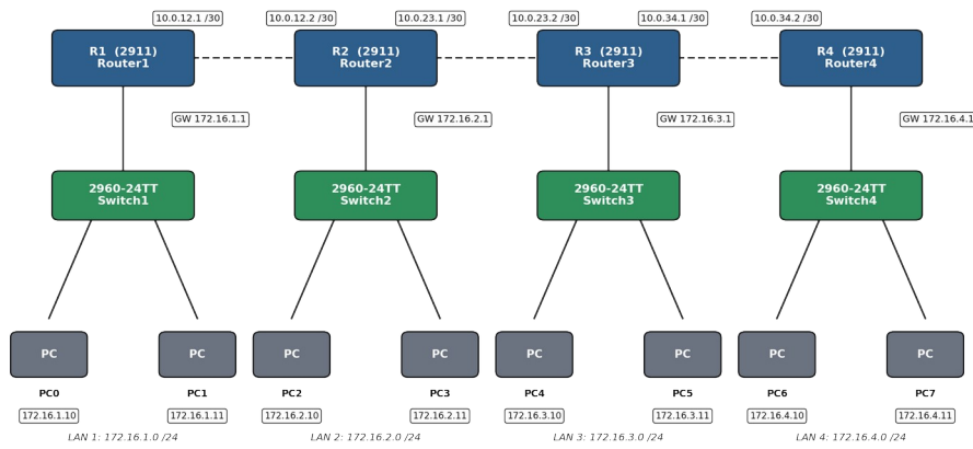
Fig 5.2 – Topology for Part B: 4 Routers, 4 Switches, 8 PCs (RIP-enabled)
