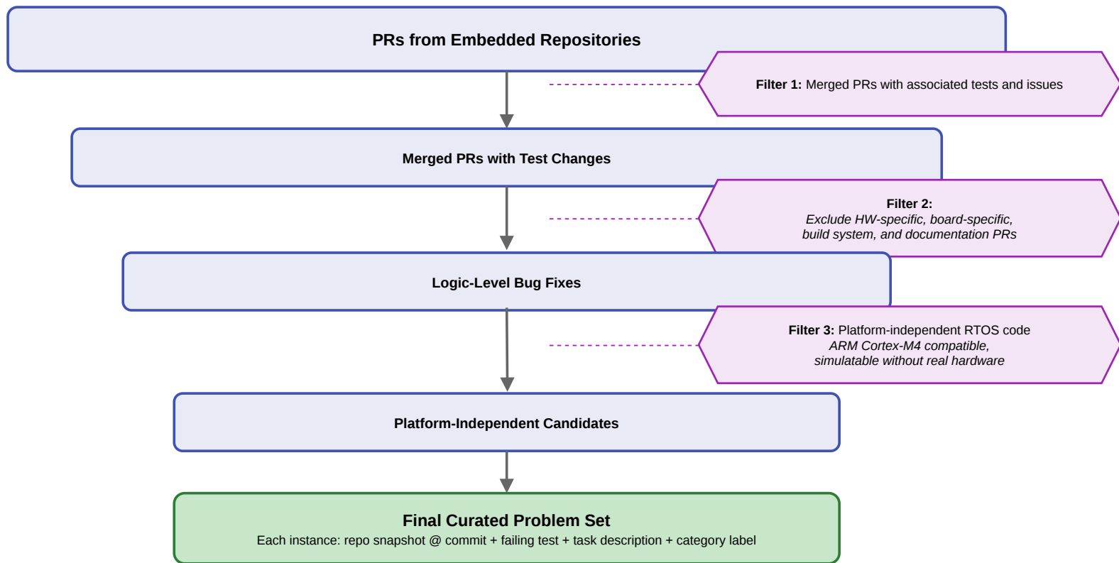
Figure 3. Problem Sourcing: PR Filtering Pipeline
