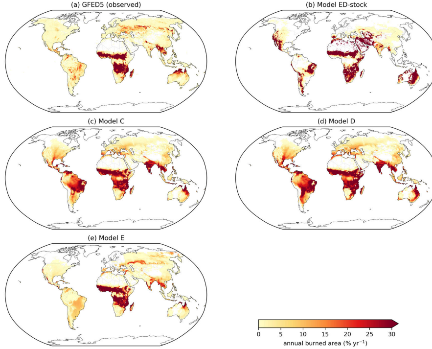
Figure 2: Mean annual burned-area fraction ( \% \text{ yr}^{-1} ) over 2001–2016 for GFED5 (observed) and the four model versions, shown on a common colour scale.
