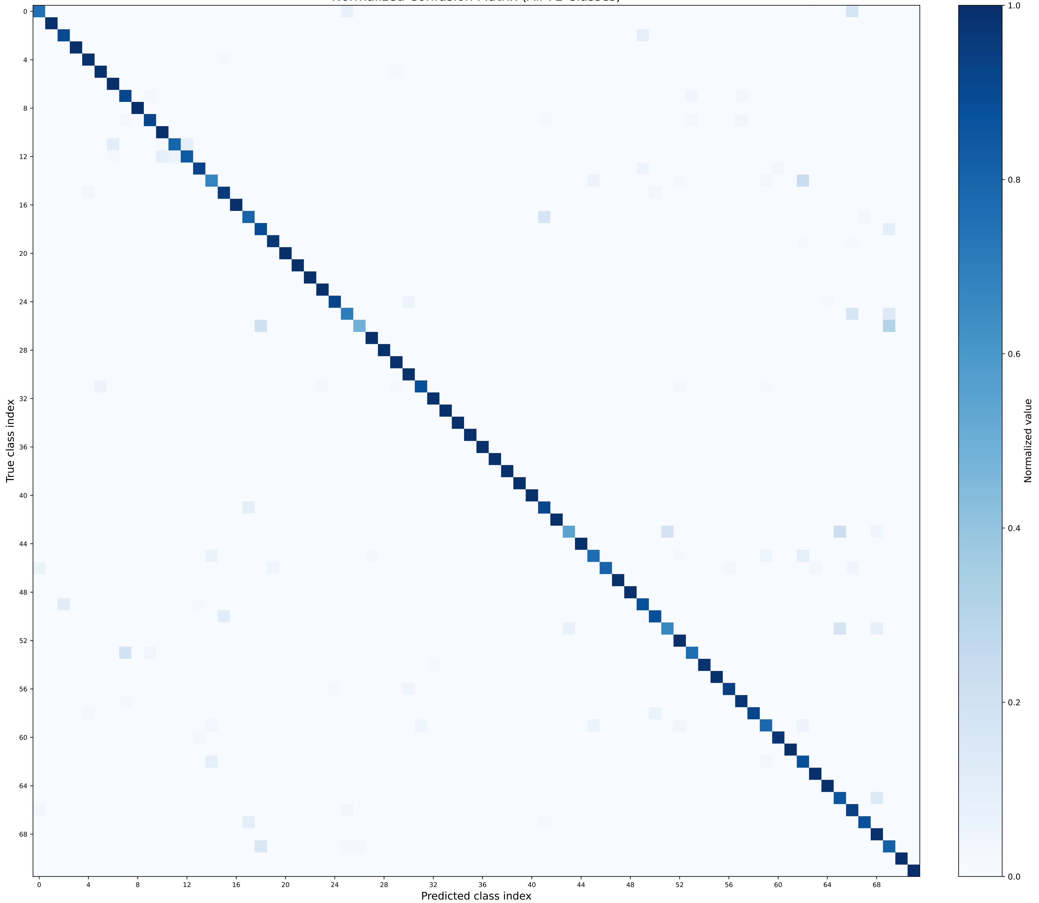
Normalized Confusion Matrix (All 72 Classes)
