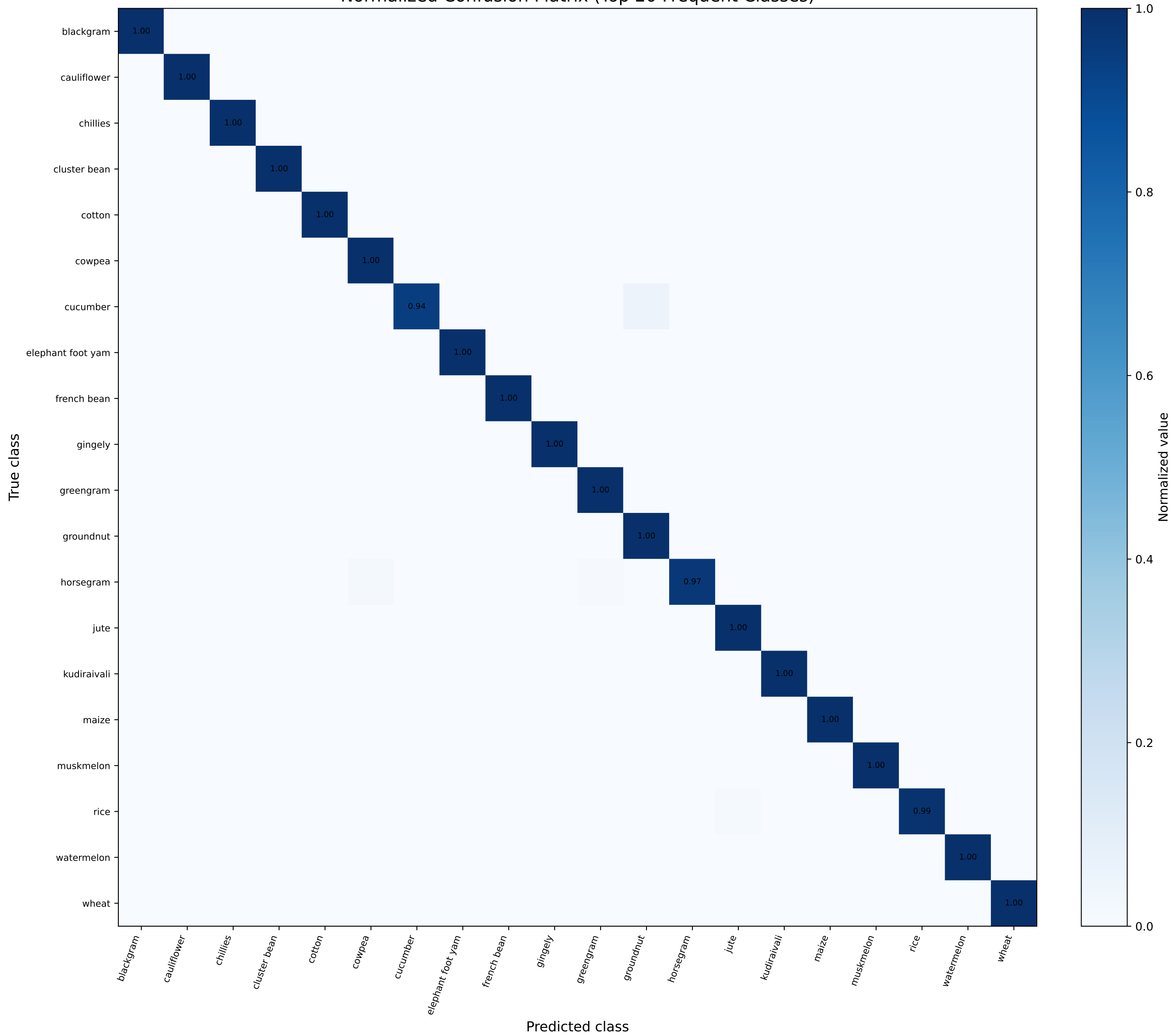
Normalized Confusion Matrix (Top 20 Frequent Classes)
