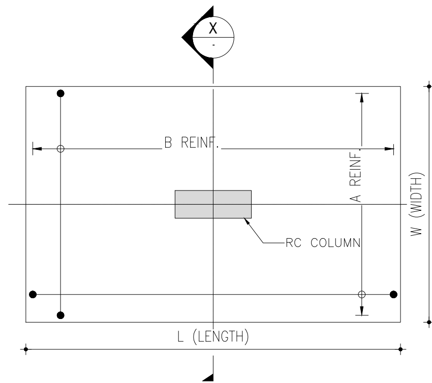
2 TYPICAL PLAN OF FOOTING SCALE 1:35
