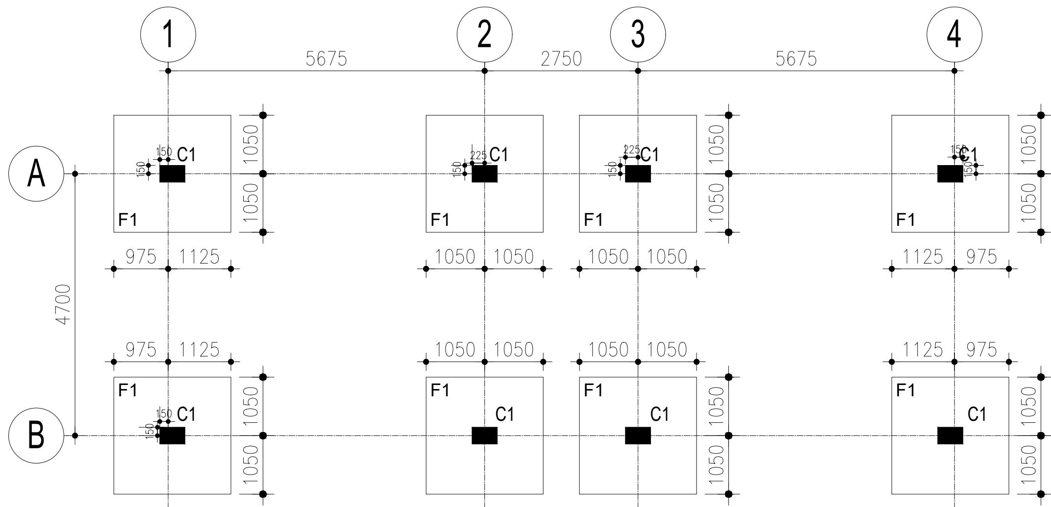
1 FOUNDATION LAYOUT SCALE 1:100
