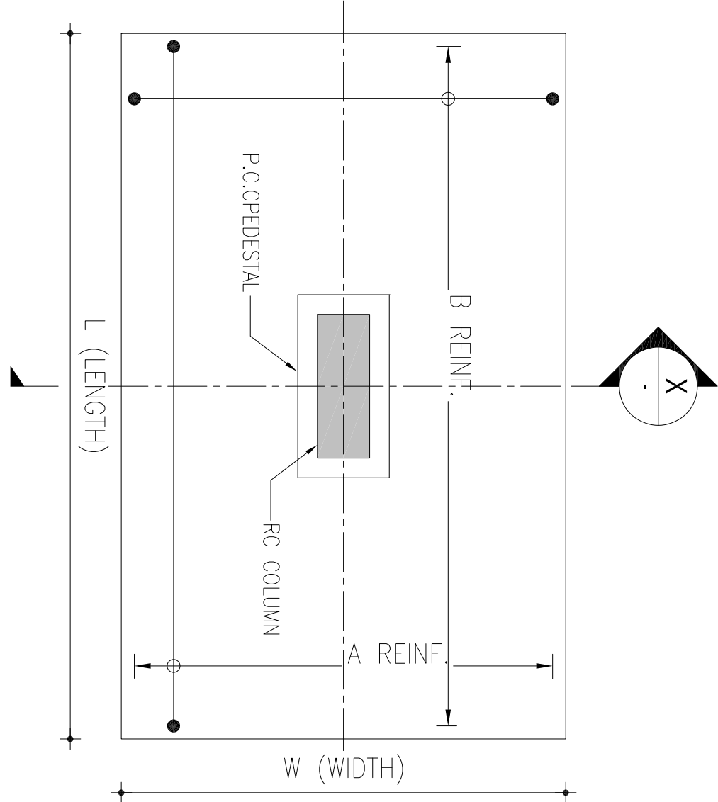
2 TYPICAL PLAN OF FOOTING
