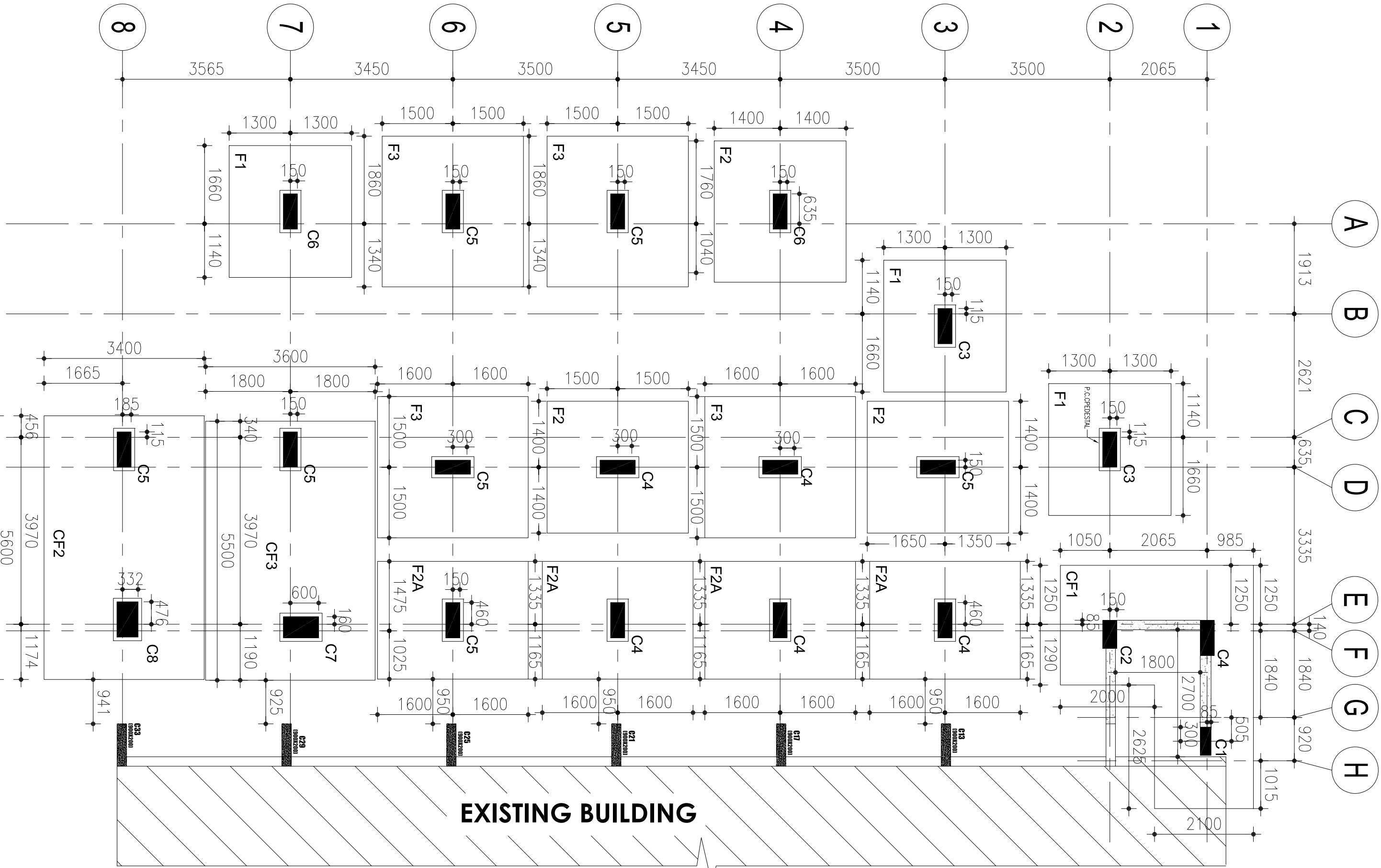
1 FOUNDATION LAYOUT
