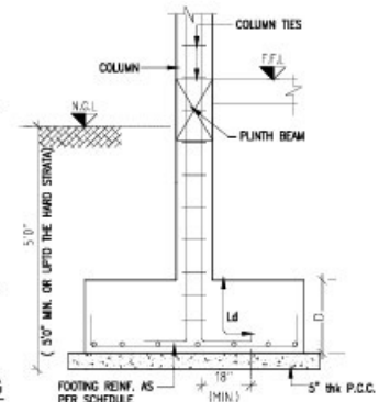
3 SECTION X SCALE 1:25
