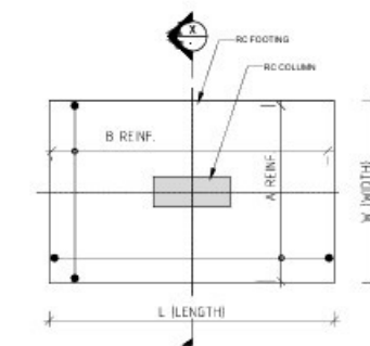
2 TYPICAL PLAN OF FOOTING SCALE 1:25 (FOR DIMENSIONS REFER TO FOOTING SCHEDULE)
