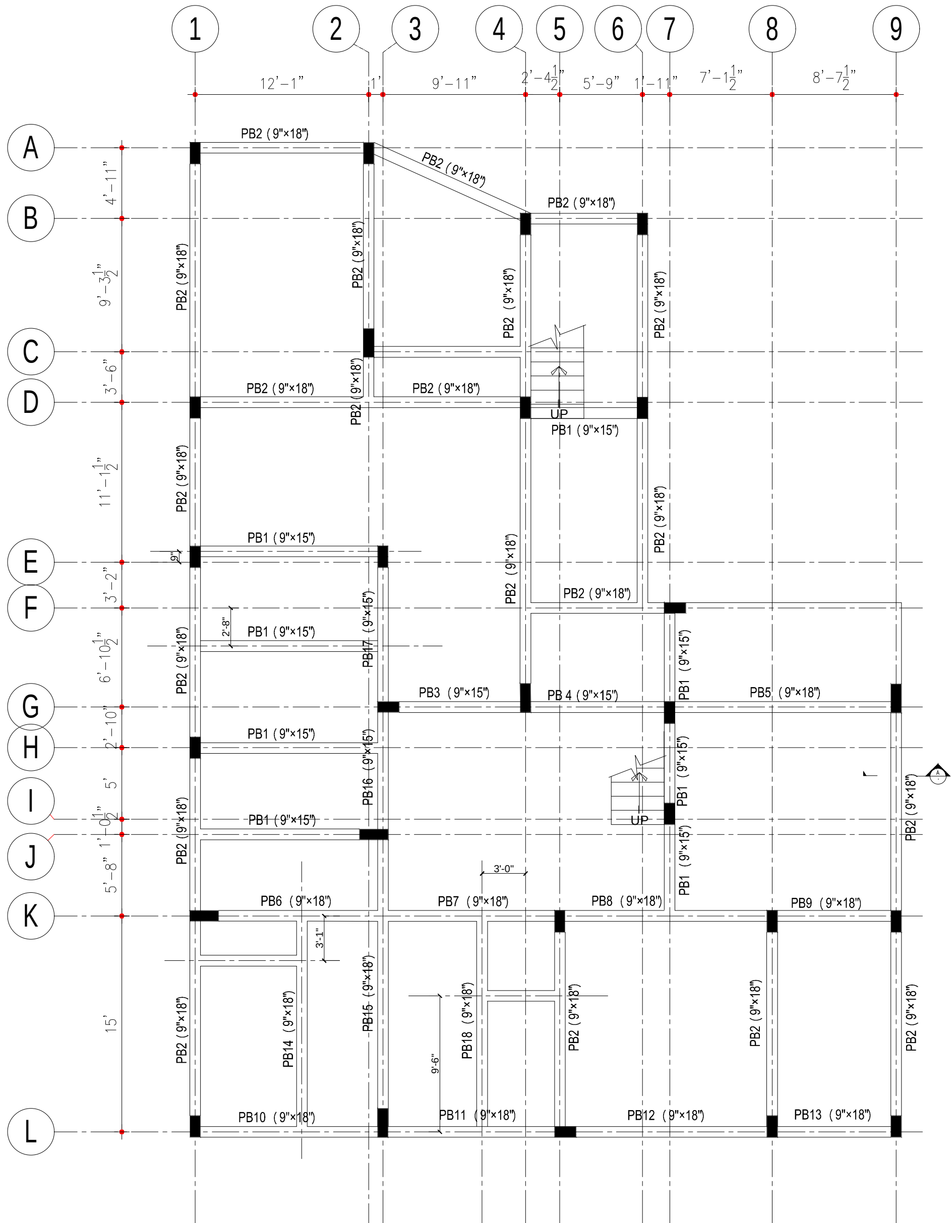
1 PLINTH BEAM LAYOUT SCALE 1:75
