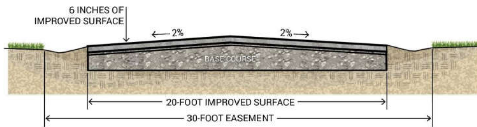
Figure 8-3-11-1 Private Road Minimum Construction Standards for Properties Outside and Inside an Area of City Impact
