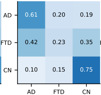
P5×functional F1=0.50
