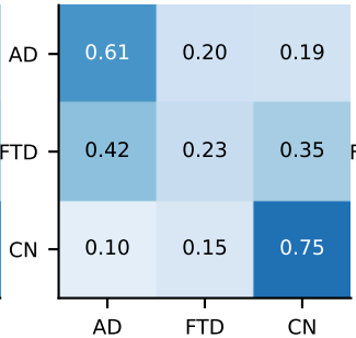
P5×functional F1=0.50
