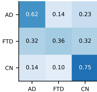
P1×spatial F1=0.56
