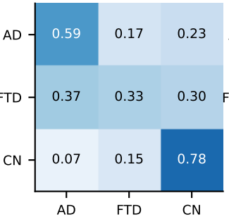
P6×functional F1=0.56
