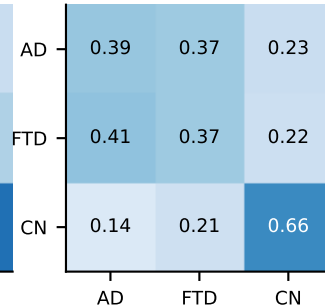
P2×functional F1=0.45
