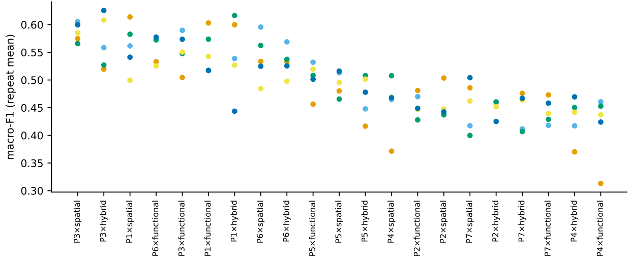
Figure S1: Mean macro-F1 of each repeat (seed) for every cell on the selection folds: variation due to the cross-validation partition and initialisation.
