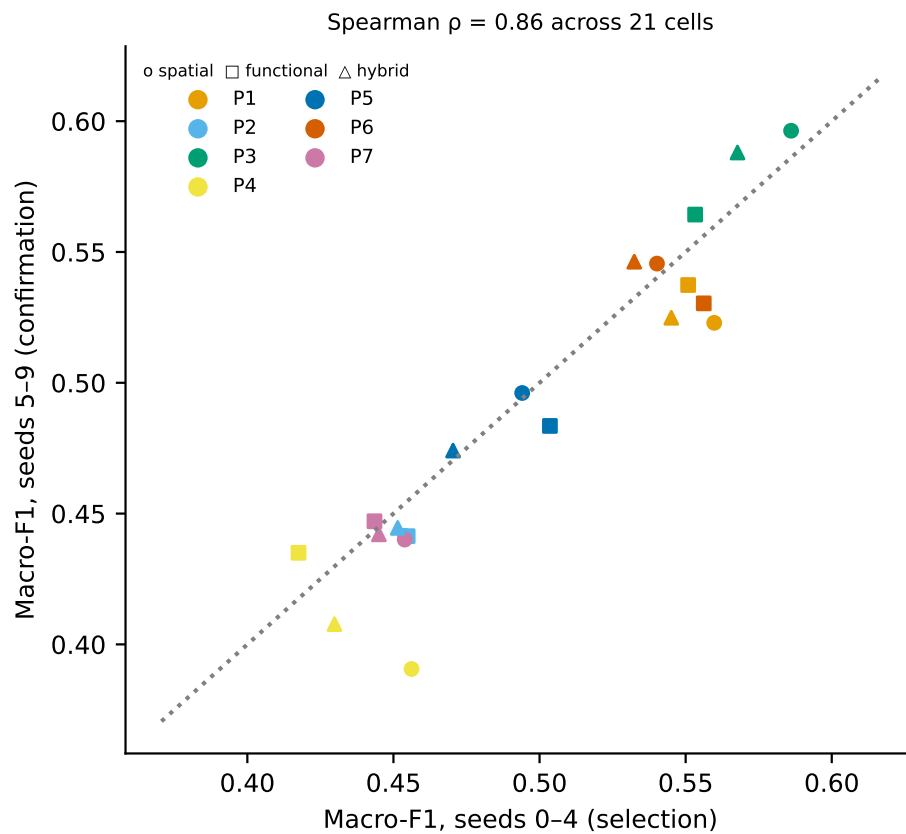
Figure S2: Every cell's mean macro-F1 on the selection folds (seeds 0–4) against the independent confirmation folds (seeds 5–9); dashed line, identity. Rank correlation: Spearman \rho = 0.86 .
