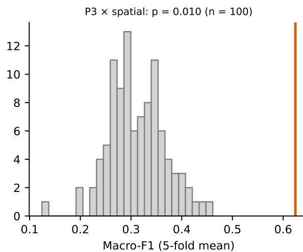
Figure S3: Label-permutation null distribution (100 permutations, first confirmation repeat's five folds) for the best cell; red line, observed macro-F1 on the same splits.
