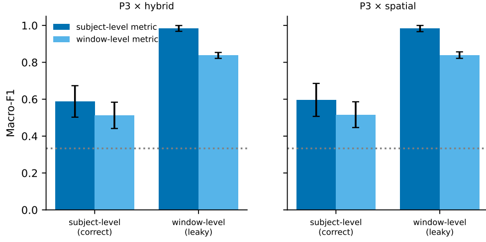
Figure 10: The same pipeline evaluated with subject-level (correct) and window-level (leaky) splitting on the confirmation folds. Bars: mean \pm SD over 25 splits; dotted line, 1/3.
