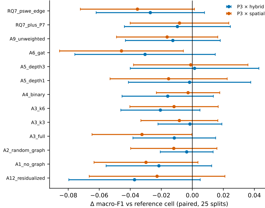
Figure 9: Ablations on the confirmation folds as paired differences from the two reference cells (mean and 95% CI over 25 splits). An asterisk would mark Nadeau–Bengio–Holm p < 0.05 ; none qualifies.
