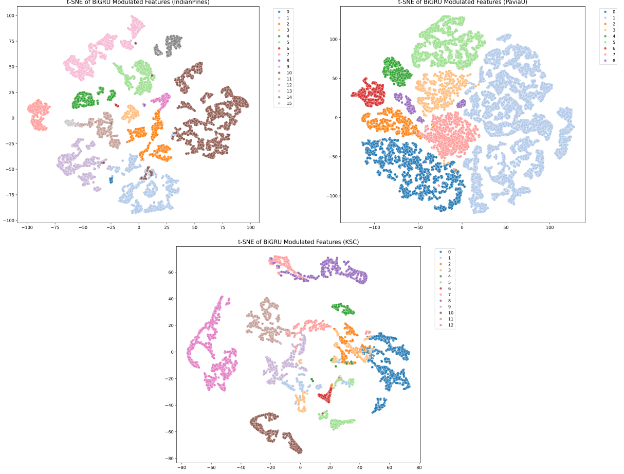
Fig. 5: Feature Separability (t-SNE) for all datasets. The strong inter-class separability supports the efficacy of the PLCWT and SMCNN processing.
