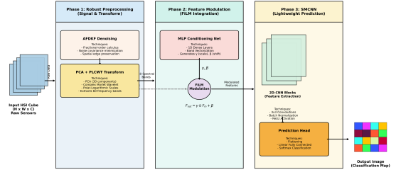
Fig. 1: End-to-End Architecture Flowchart of the SMCNN-MLP Framework.
