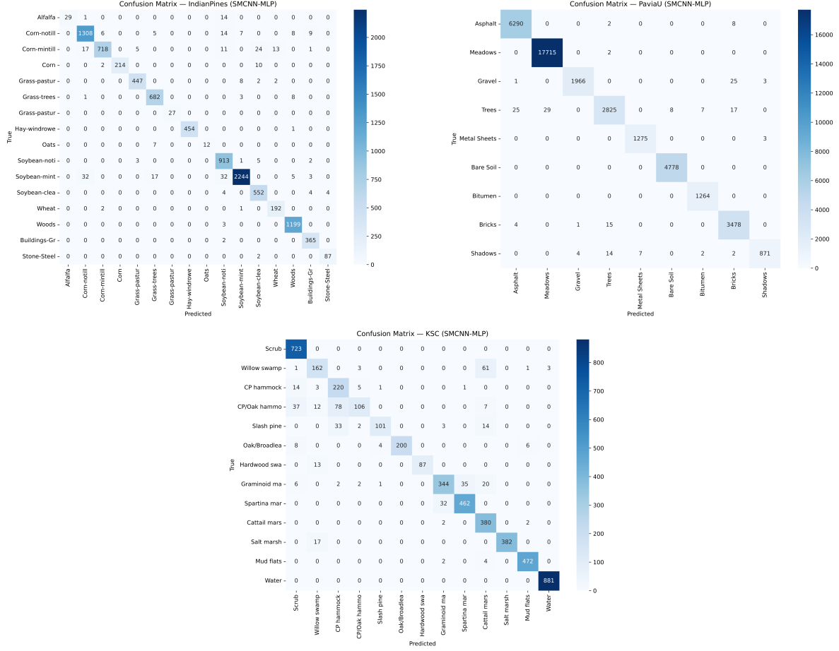
Fig. 9: Confusion Matrices for all datasets. Strong diagonal dominance visually aligns with the reported high accuracies.
