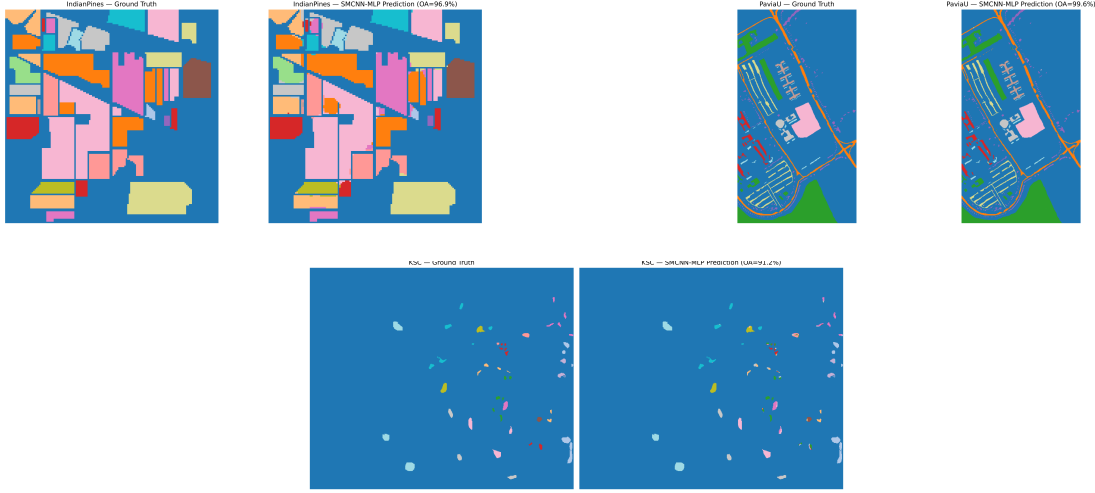
Fig. 8: Full Classification Maps for (a) Indian Pines, (b) PaviaU, and (c) KSC datasets. Sharp boundaries suggest effective AFDFK spatial edge preservation.
