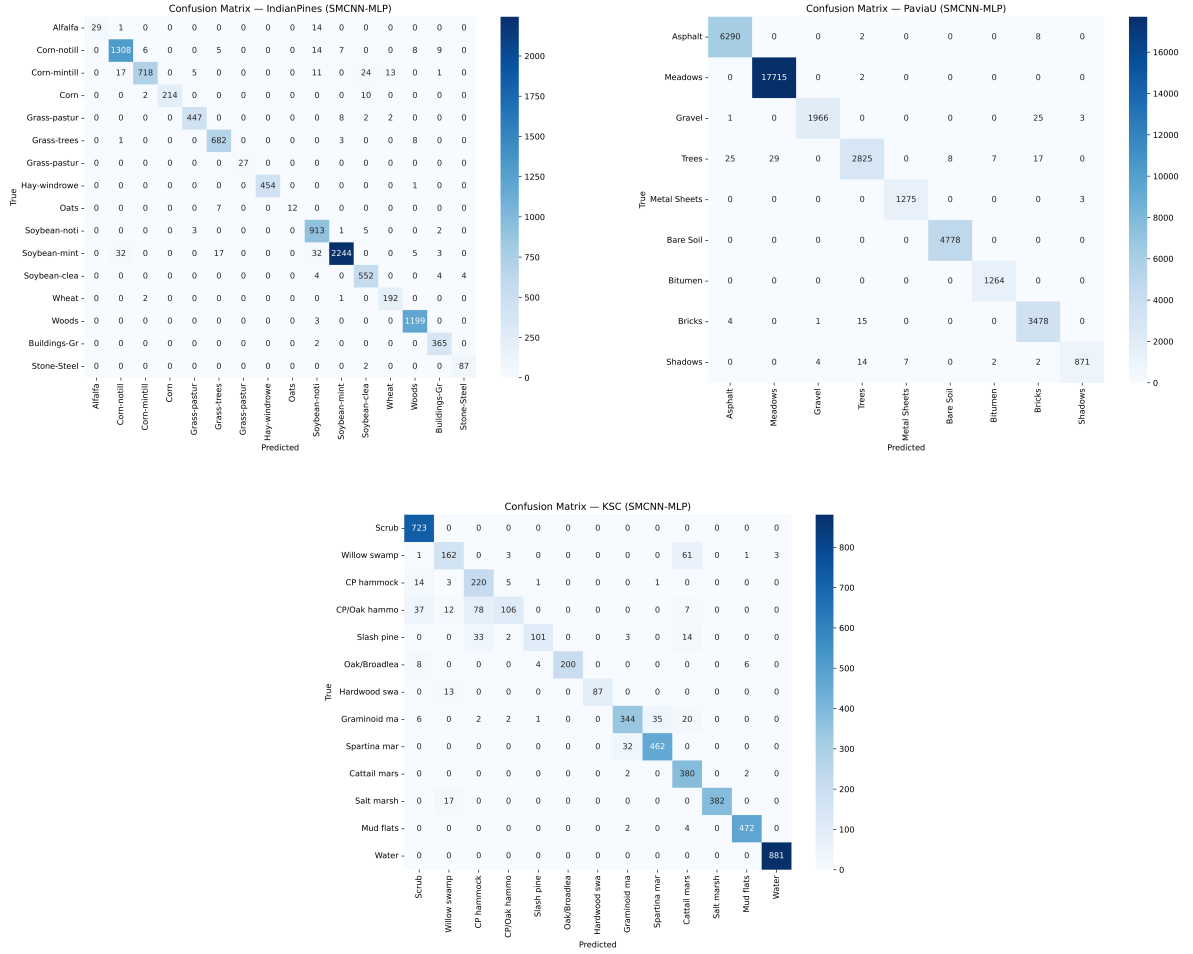
Fig. 7: Confusion Matrices for (a) IndianPines, (b) PaviaU, and (c) KSC datasets. Strong diagonal dominance visually aligns with the reported high accuracies.
