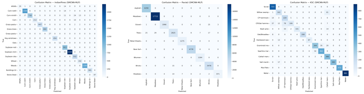
Fig. 9: Confusion Matrices for all datasets. Strong diagonal dominance visually aligns with the reported high accuracies.
