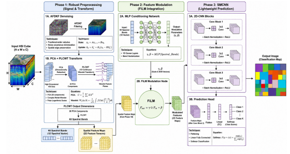
Fig. 1: End-to-End Architecture Flowchart of the SMCNN-MLP Framework.
