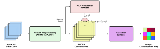
Fig. 1: End-to-End Architecture Flowchart of the SMCNN-MLP Framework.
