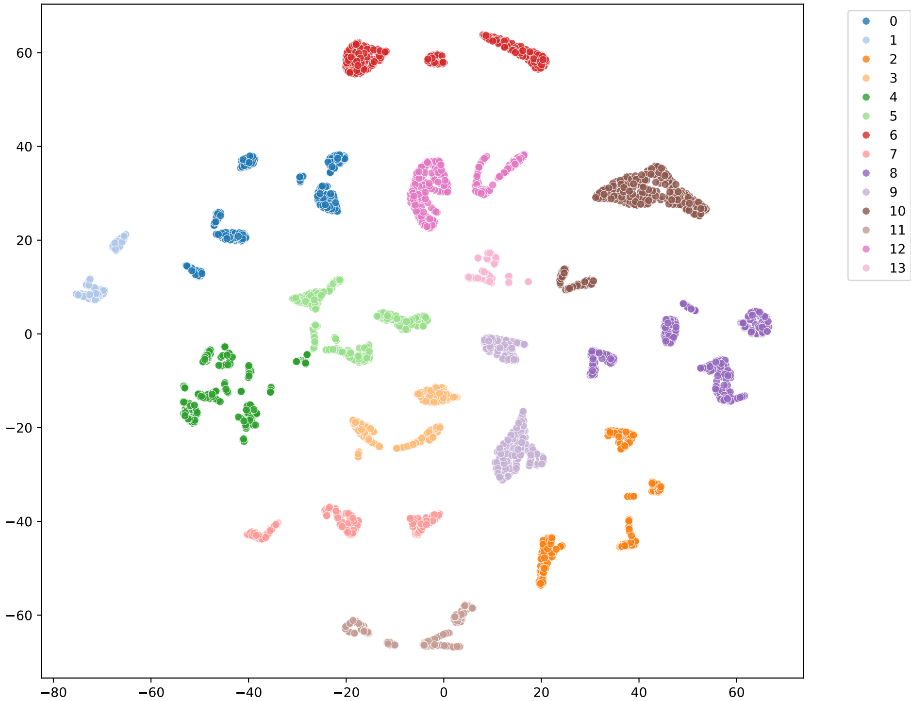
t-SNE of BiGRU Modulated Features (Botswana)
