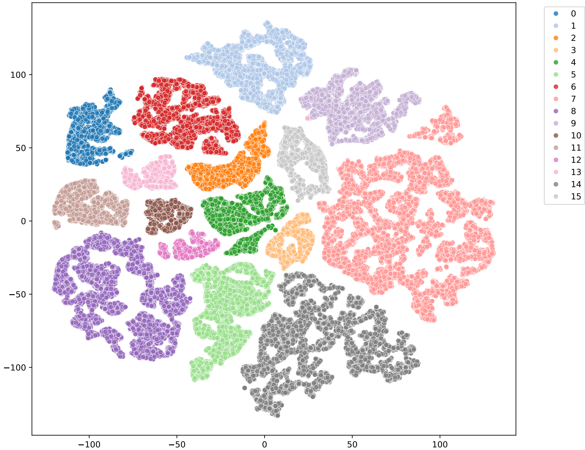
t-SNE of BiGRU Modulated Features (Salinas)
