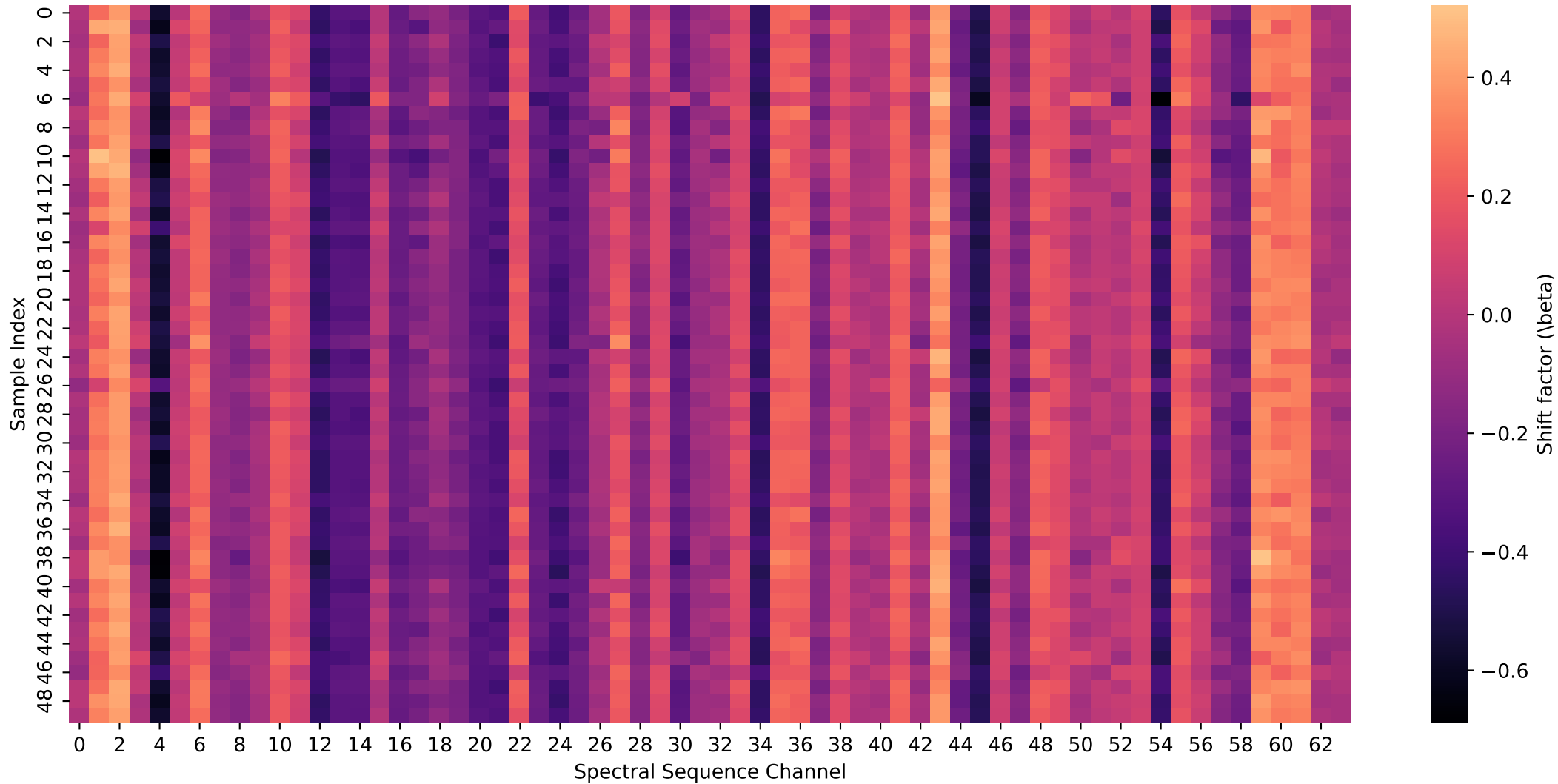
WHU_Hi BiGRU Shift ( \beta )
