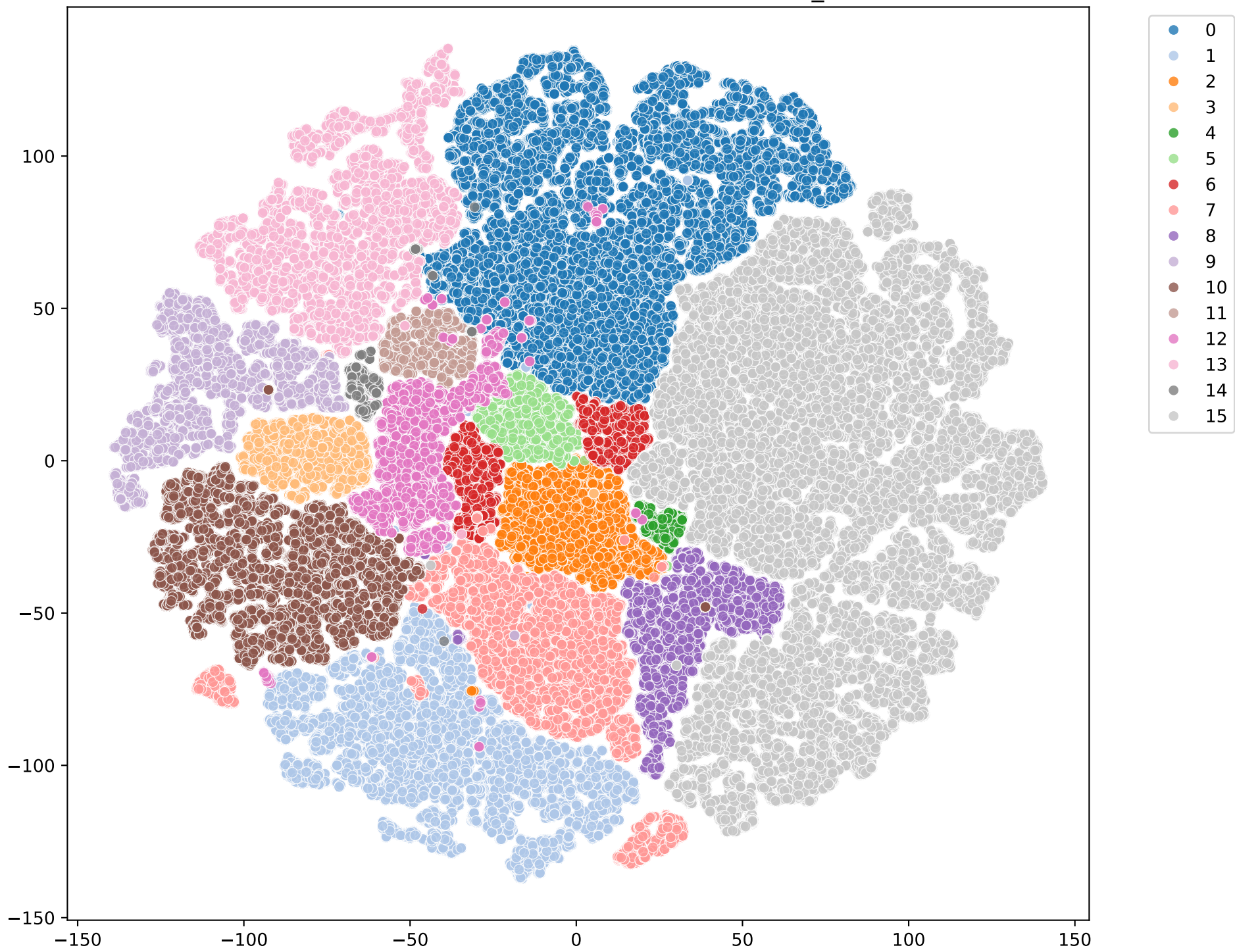
t-SNE of BiGRU Modulated Features (WHU_Hi)
