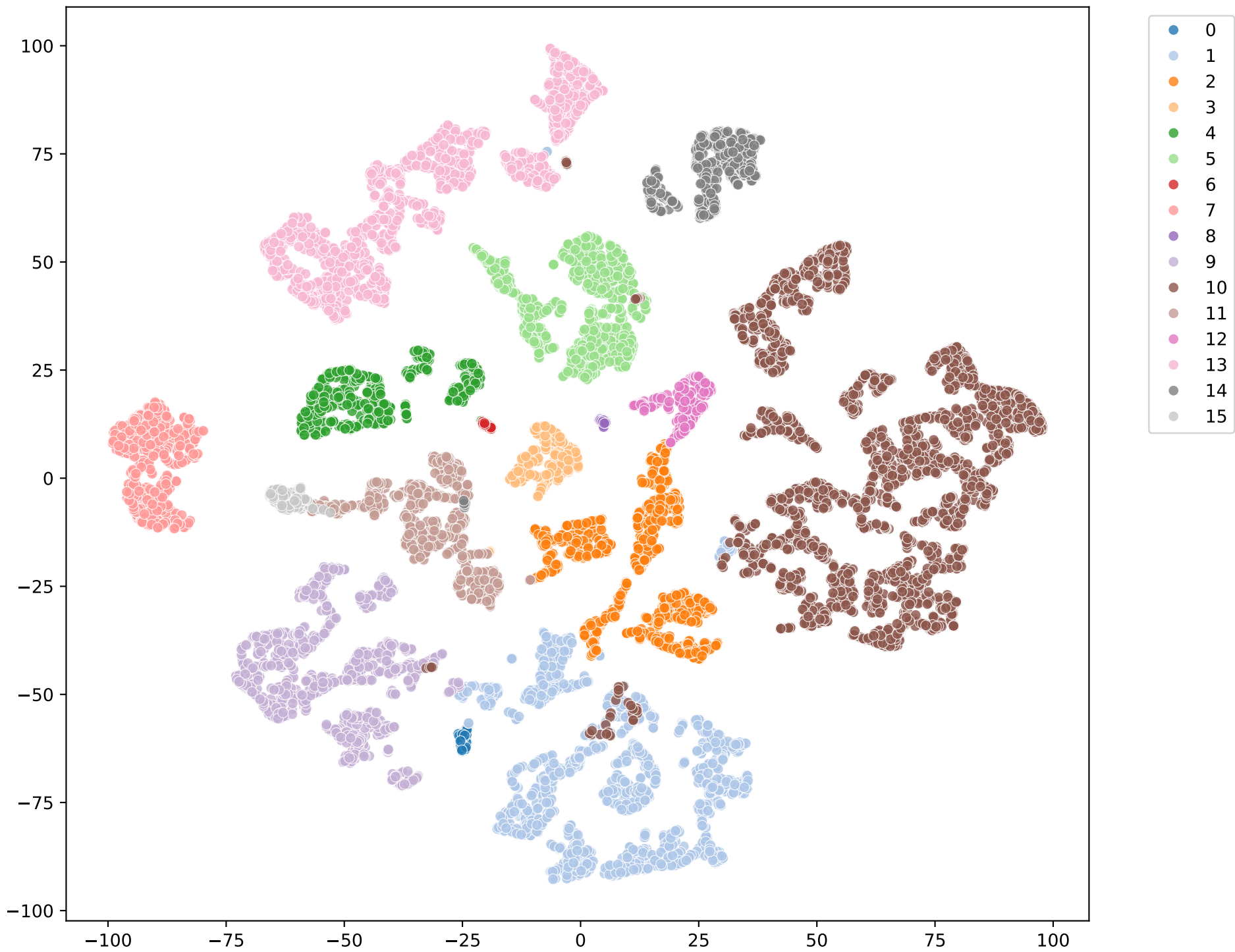
t-SNE of BiGRU Modulated Features (IndianPines)
