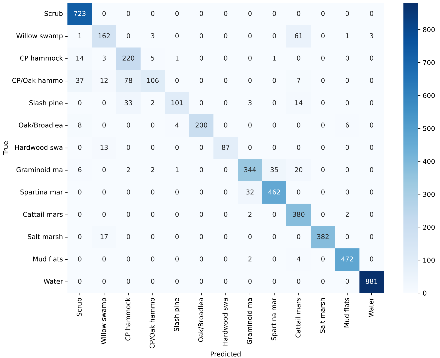
Confusion Matrix — KSC (SMCNN-MLP)
