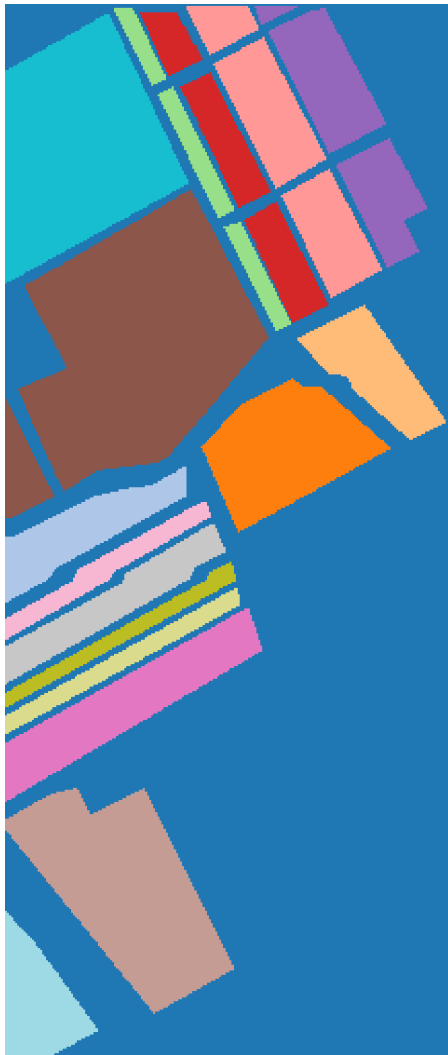
Salinas — Ground Truth
