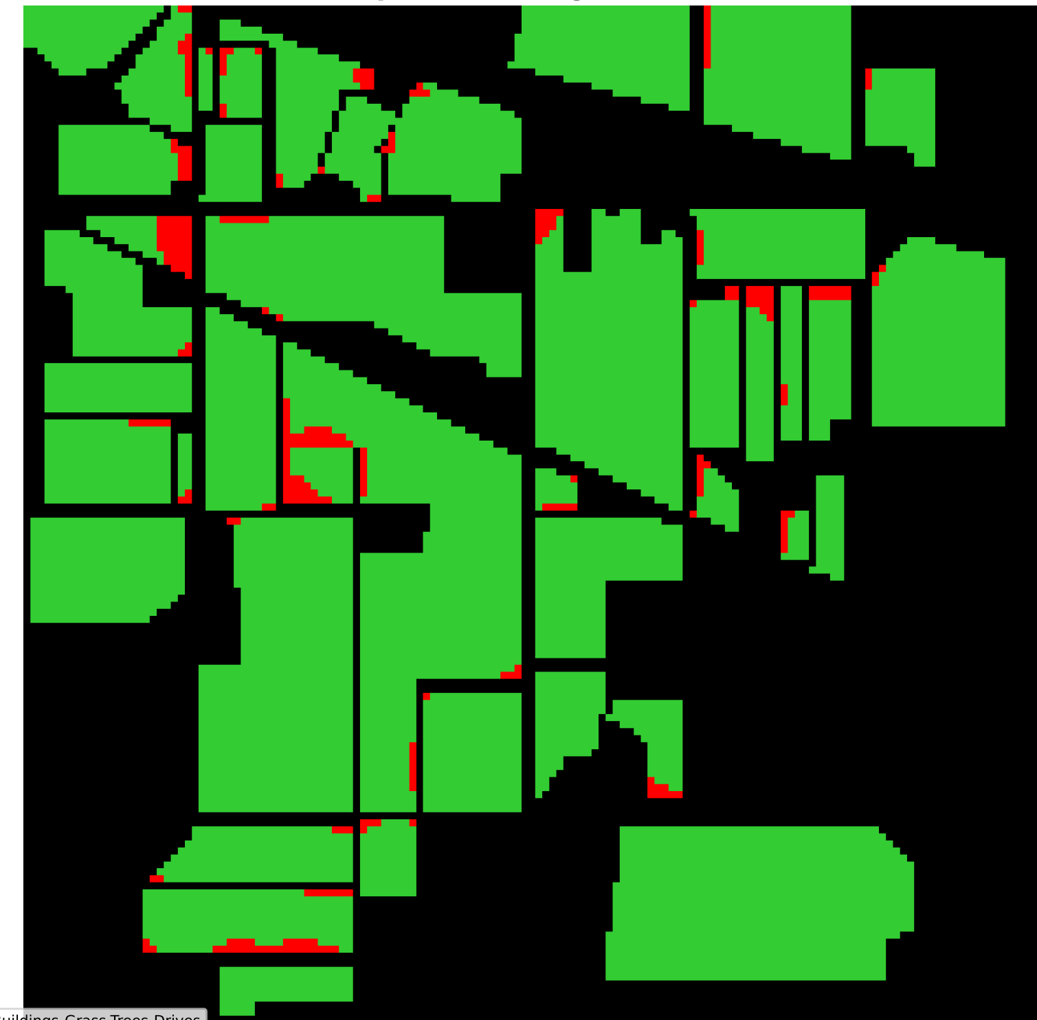
Error Map (Red=Wrong) — IndianPines
