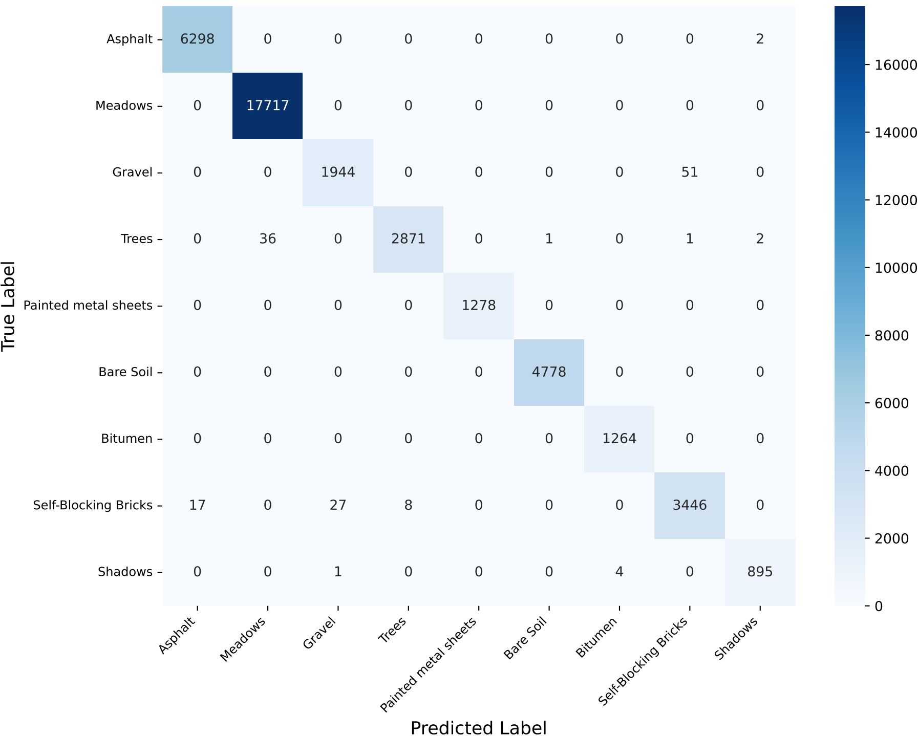
Confusion Matrix — PaviaU
