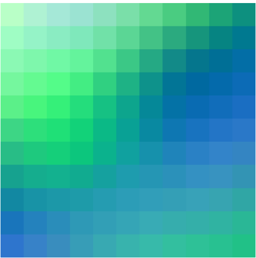
True: Gravel
