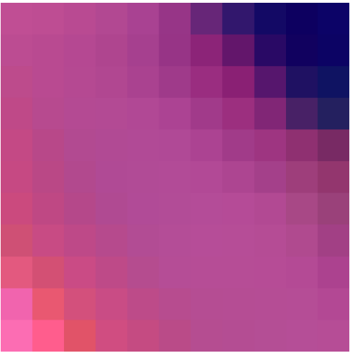
True: Trees
