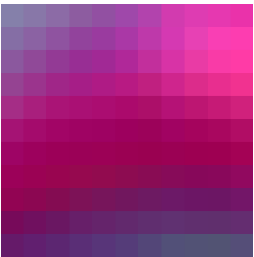
True: Meadows
