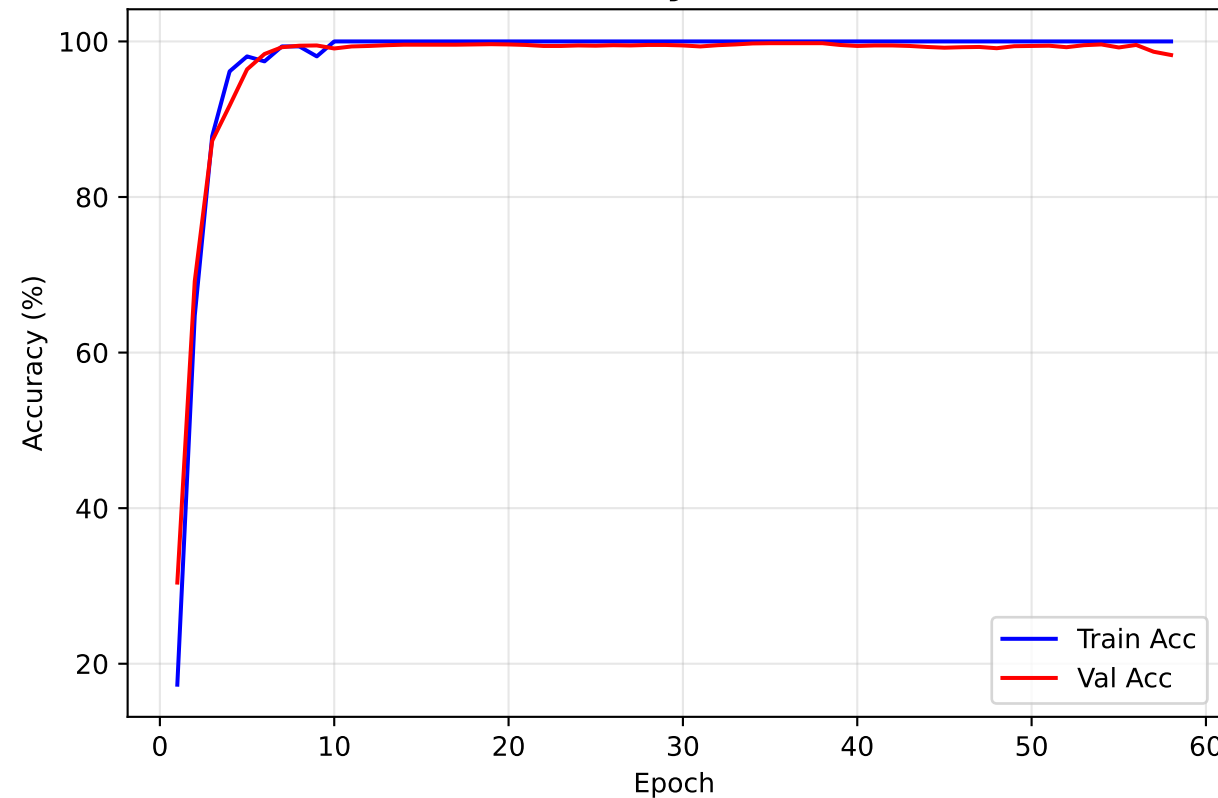
Accuracy Curves
