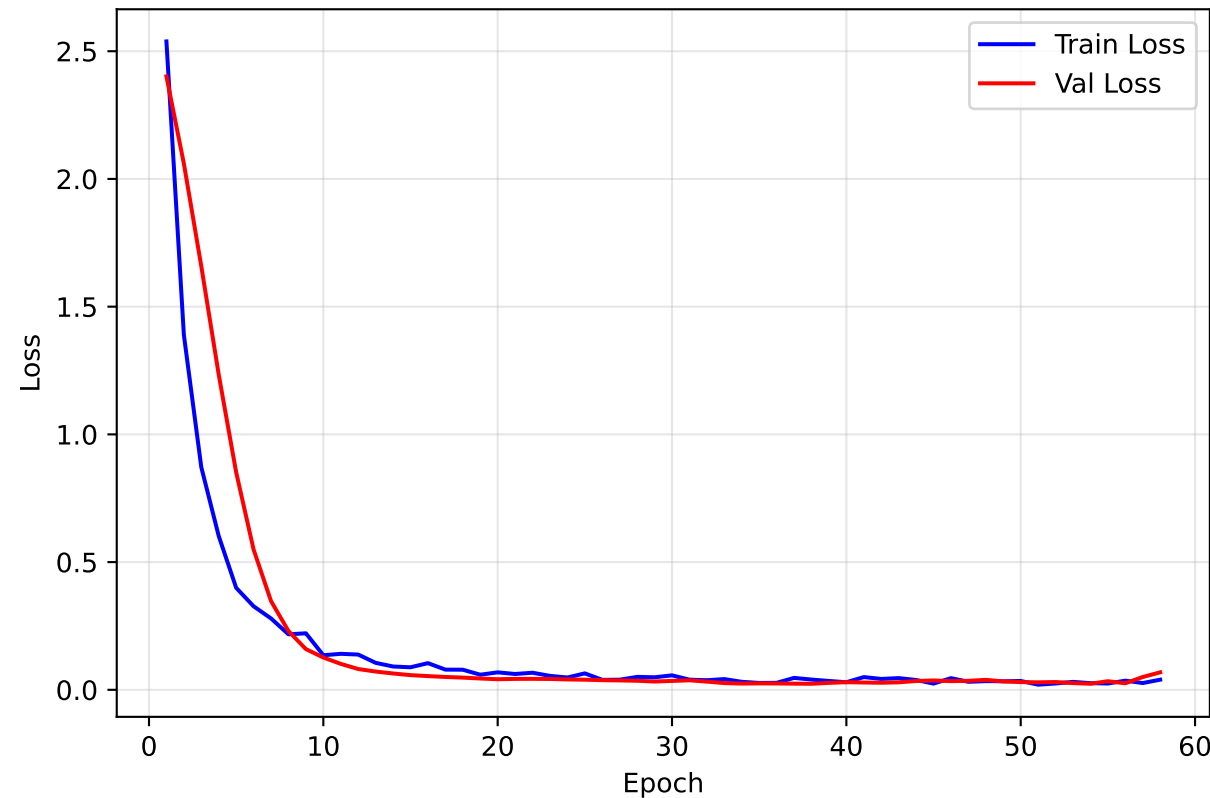
Loss Curves
