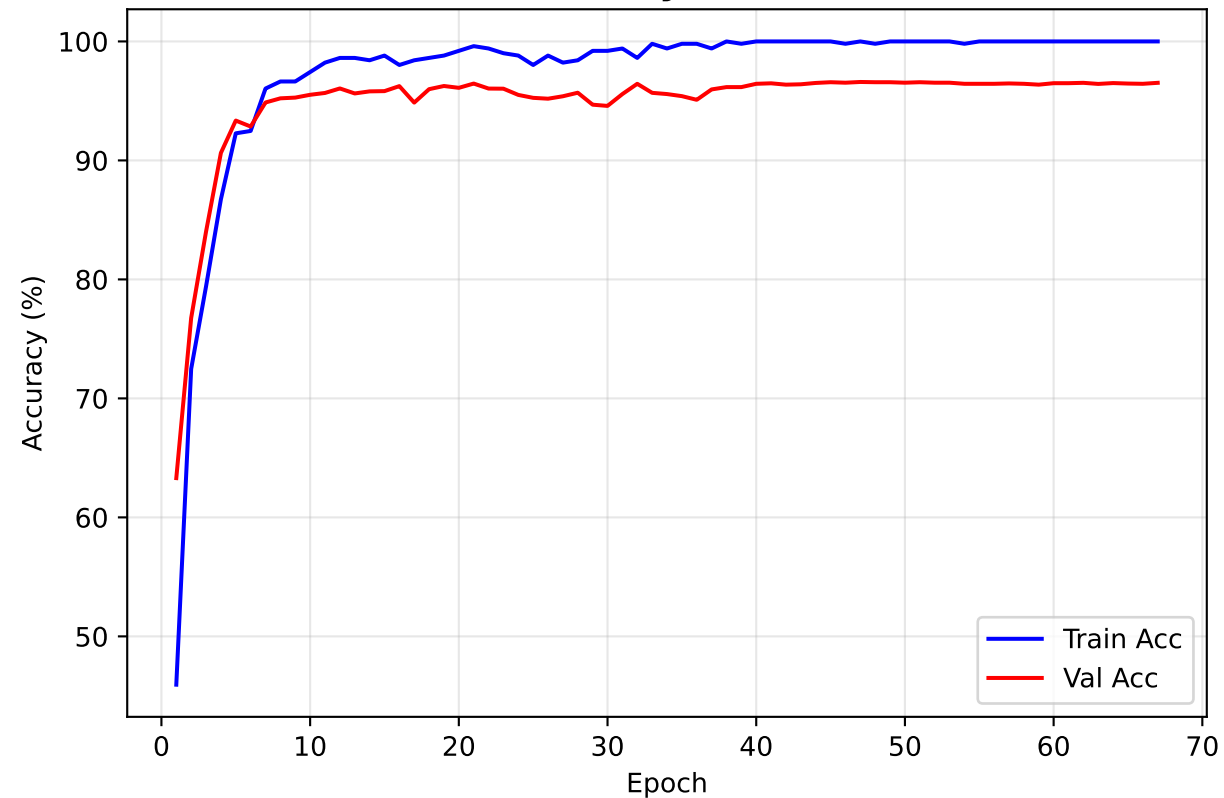
Accuracy Curves
