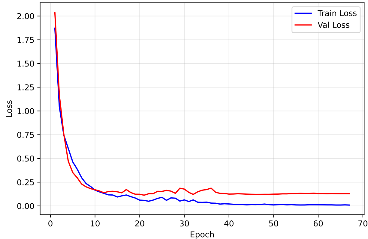
Loss Curves
