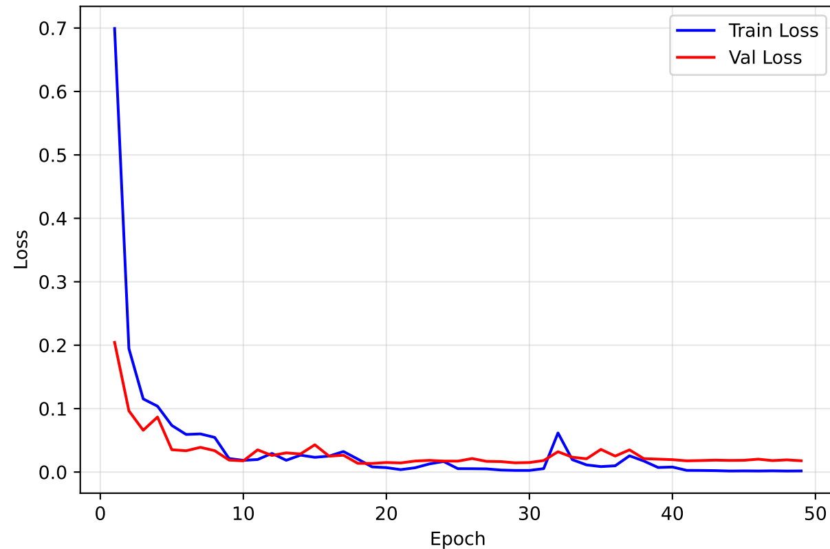
Loss Curves
