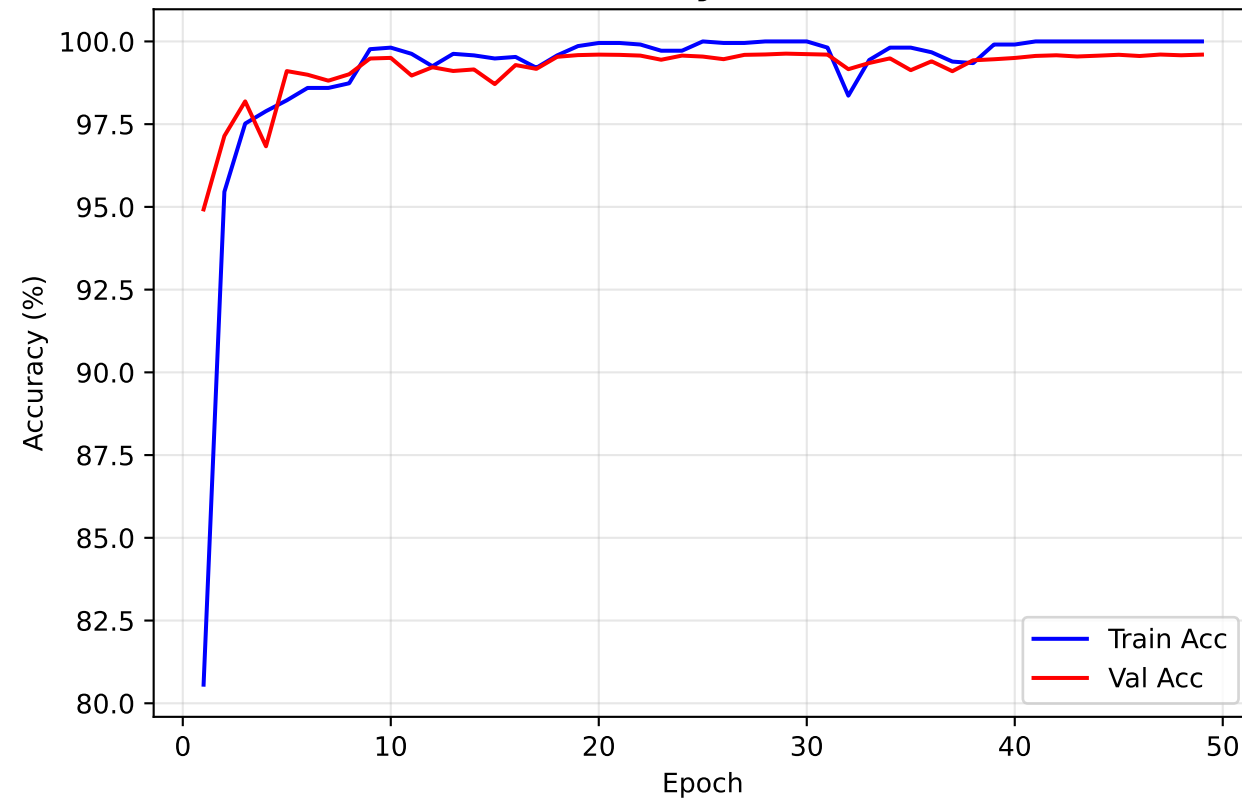
Accuracy Curves
