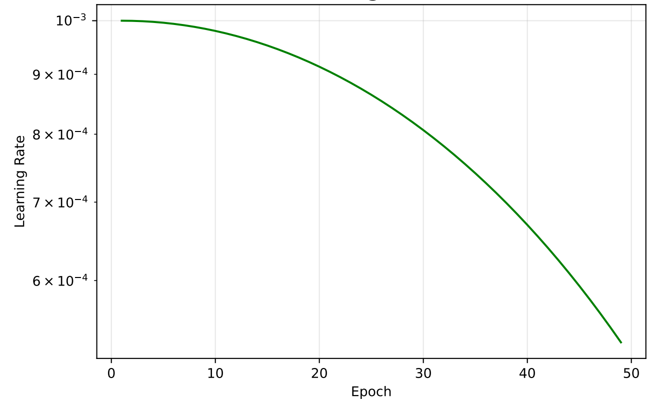
SFWOA Learning Rate Schedule
