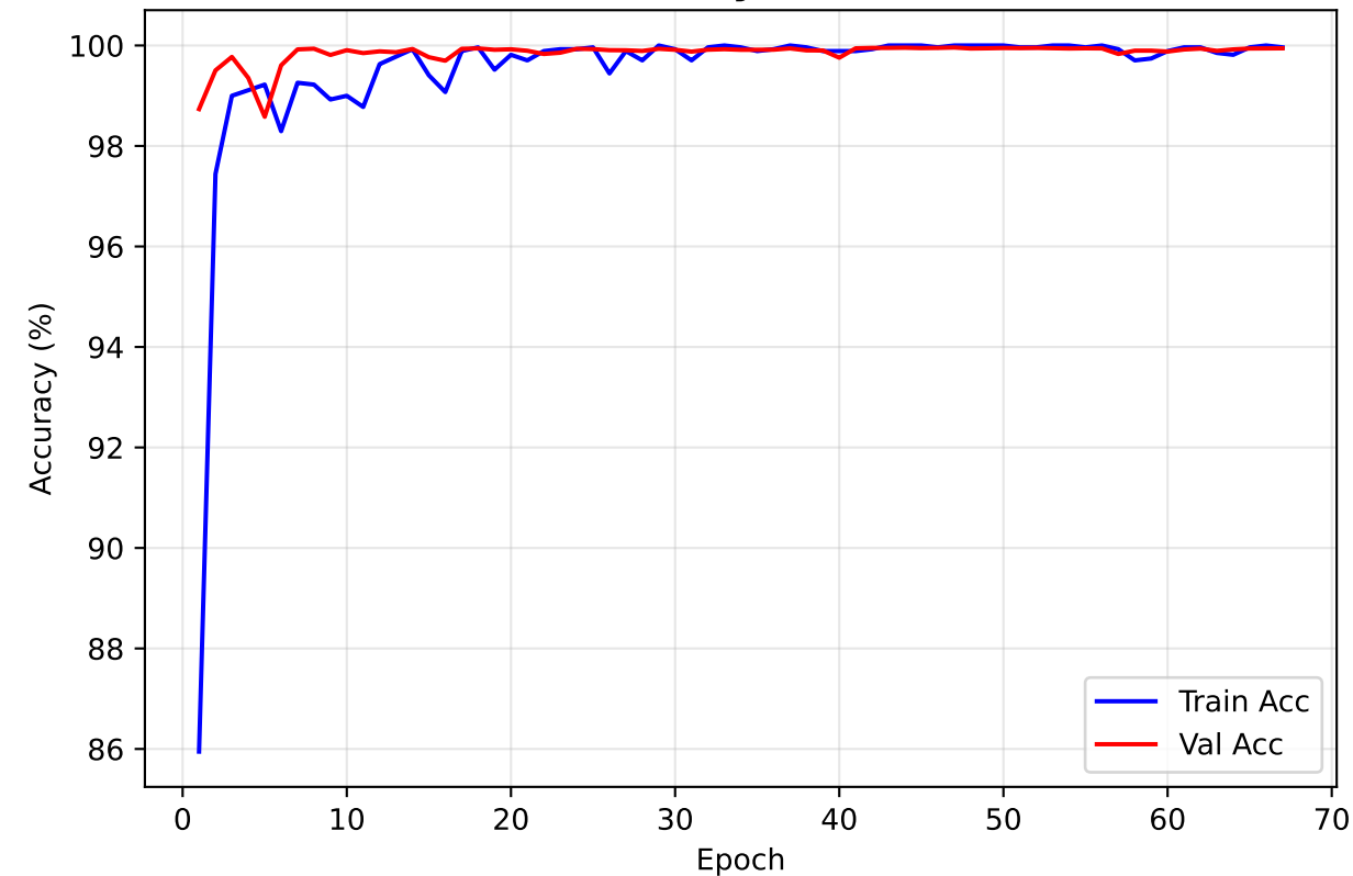
Accuracy Curves
