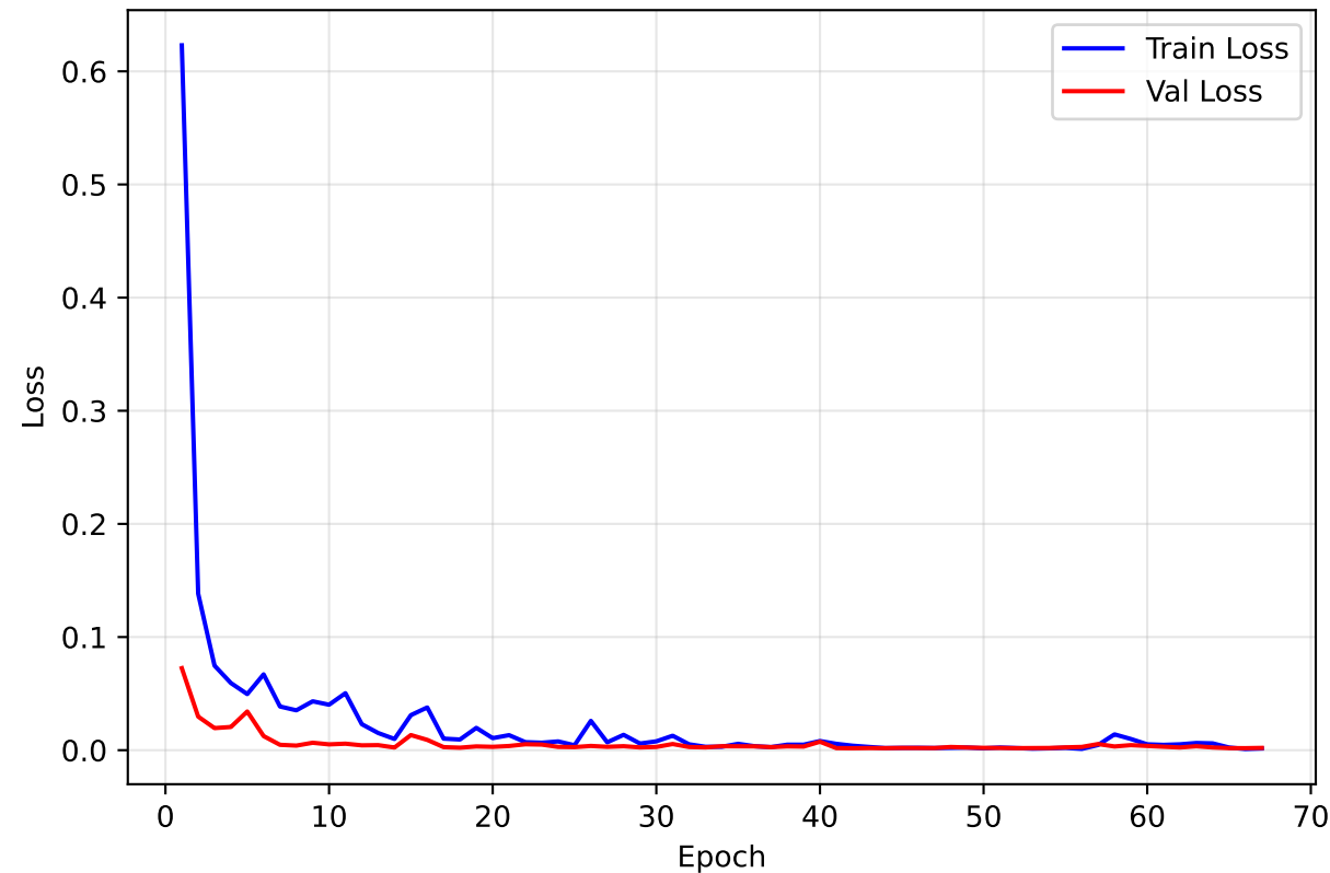
Loss Curves
