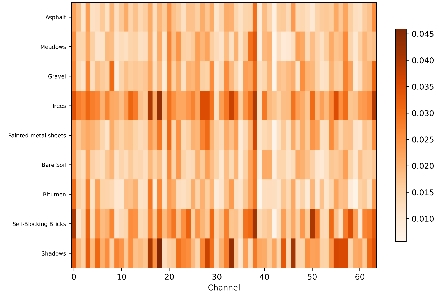
\gamma Std Dev (input-dependent)
