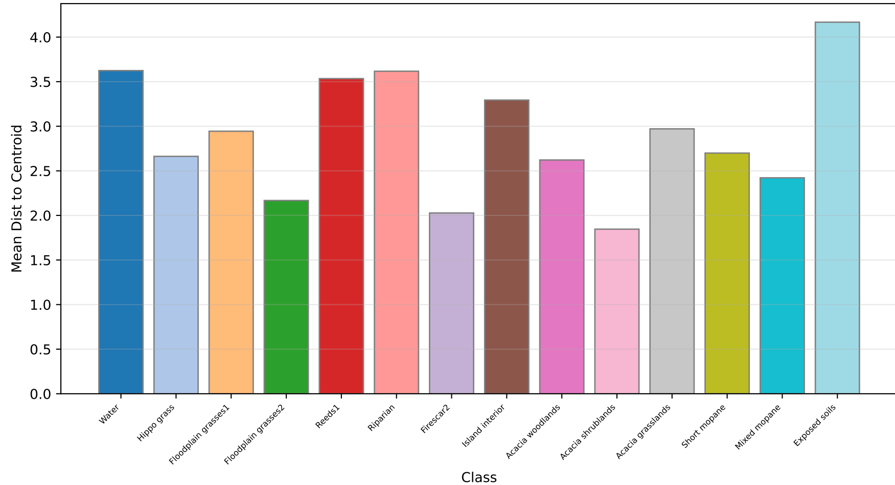
Intra-Class Compactness Fisher = 16.26
