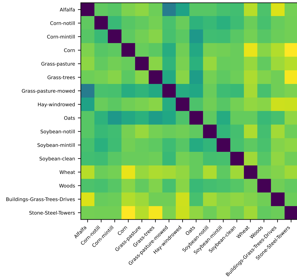
Inter-Class Distance
