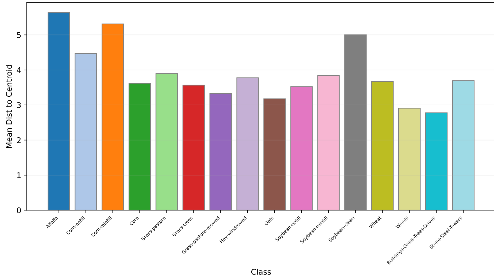
Intra-Class Compactness Fisher = 6.69
