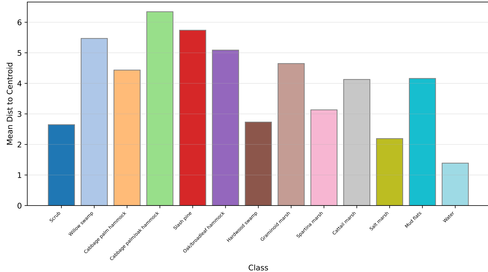
Intra-Class Compactness Fisher = 4.43
